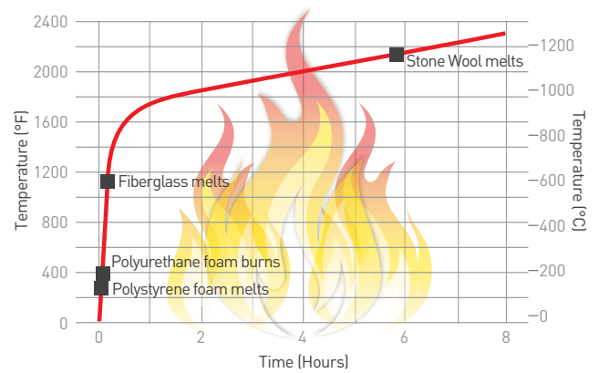
Temperature Development in a Standard Fire (ASTM E119)
